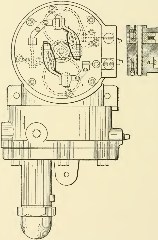
Fig. 89. Front View of Pump Governor
